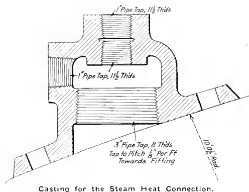
Casting for the Steam Heat Connection.
